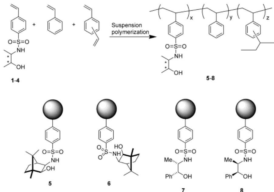
Scheme 1. Preparation of polymer-supported chiral N -sulfonylamino alcohol ligands
