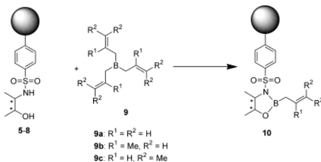
Scheme 2. Preparation of polymer-supported allylboron reagents
