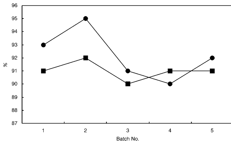
Fig. 1. Yield and enantioselectivities of the allylboration of N -silylimine 13a with multiple use of the polymer-supported chiral allylboron reagent prepared from 7b . ● % yield of 14a ; ■ % ee of 14a .
