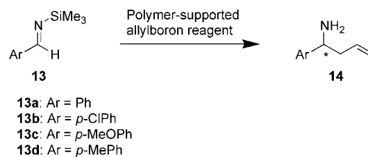
Scheme 4. Enantioselective allylboration of N -silylimines
